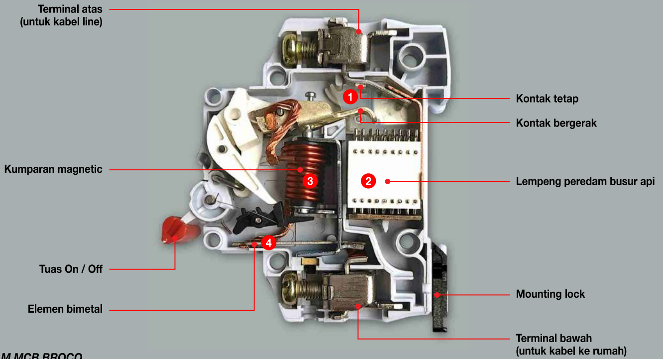
DIAGRAM MCB BROCO
