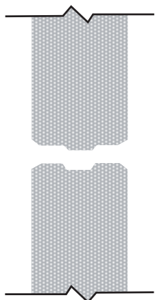
SINGLE TONGUE & GROOVE PROFILE ( 75, 100, 125mm )
