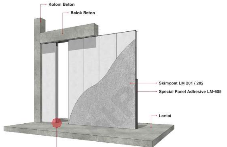
Gb. 4 Dinding Panel AAC
